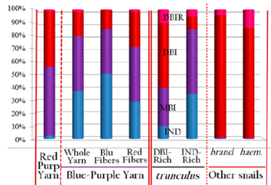
Figure 13: Relative integrated peak areas as percentages (at 288 nm) calculated from the chromatograms of the red-purple and blue-purple dyed yarns of archaeological textile KTN 1475 and compared with modern raw snail pigments; the color schemes of the identified dyes are blue for IND, violet for MBI, red for DBI, and pink for DBIR.
